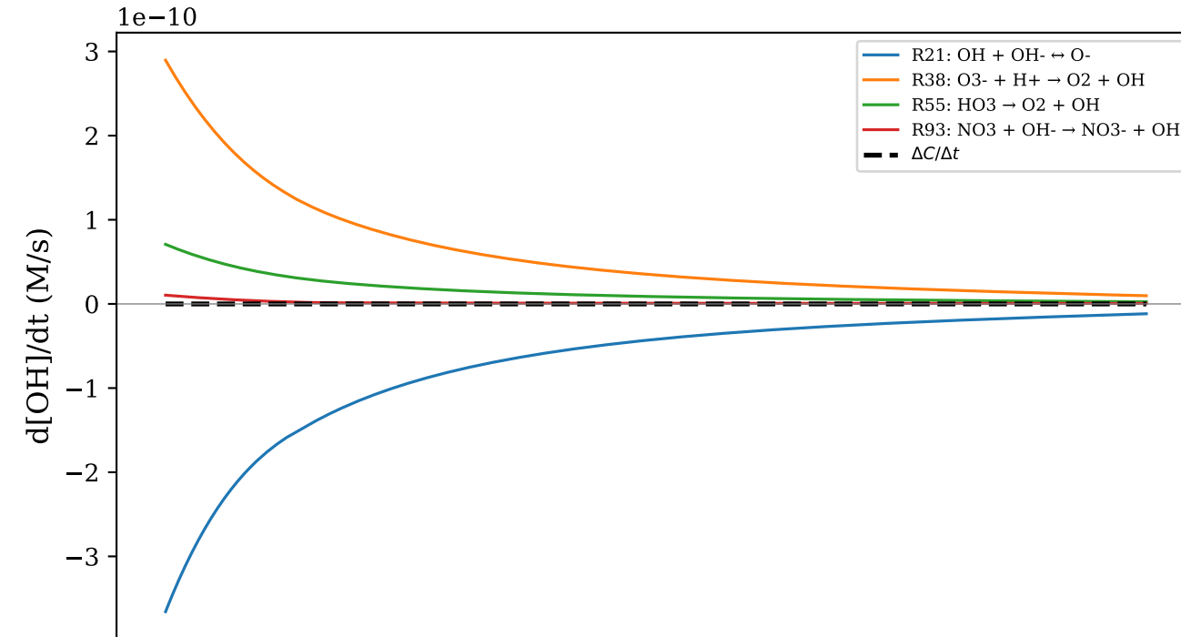
(b) OH [final=0.03 pM]
