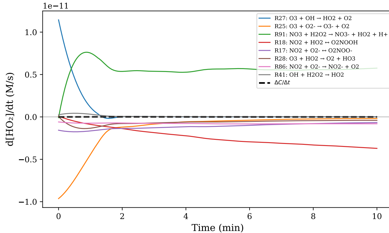
(c) HO 2 [final=0.44 pM]
